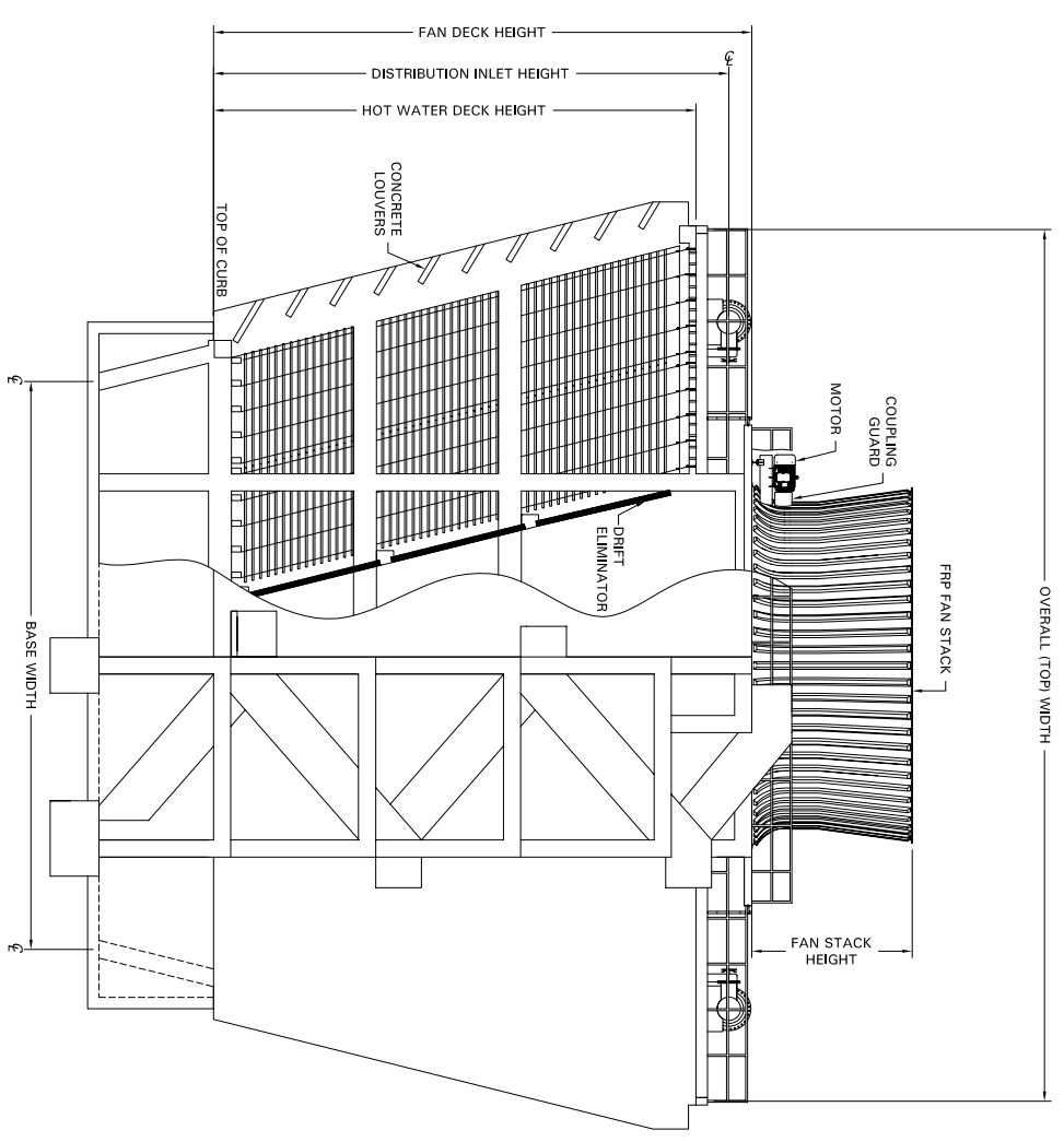
TRANSVERSE ELEVATION
